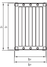
Pallet trolley with corner guards
