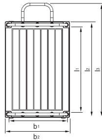
Rack trolley, low
