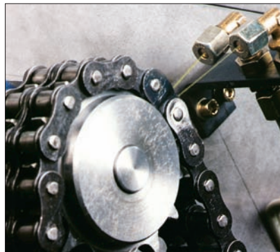
Contact-free oil application via nozzles
